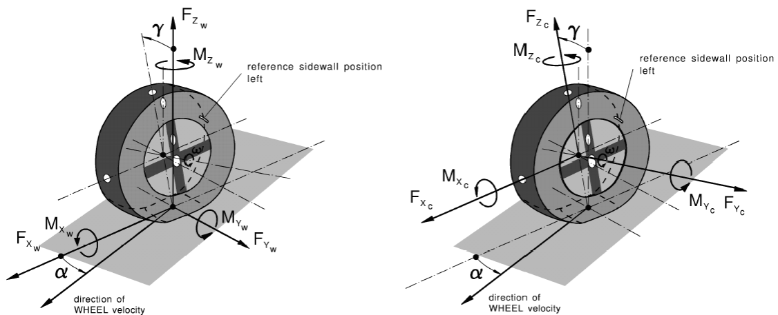
Figure 4.5: ISO sign conventions
