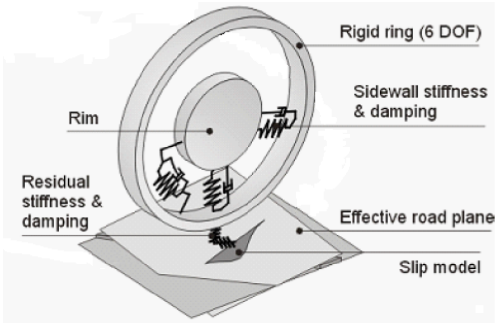
Figure 4.3: Schematic representation of MF-Tyre/MF-Swift.
